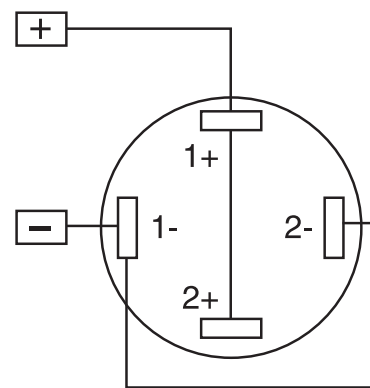
Speakon™ Connection
