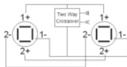
Two Way Crossover
