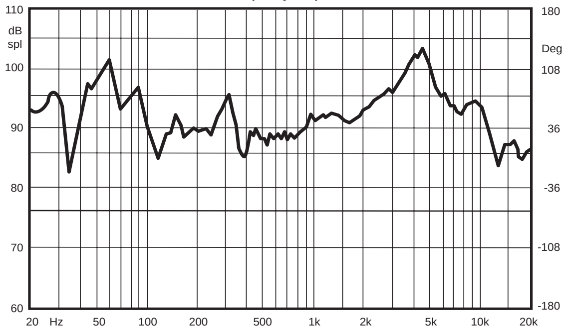
Frequency Response
